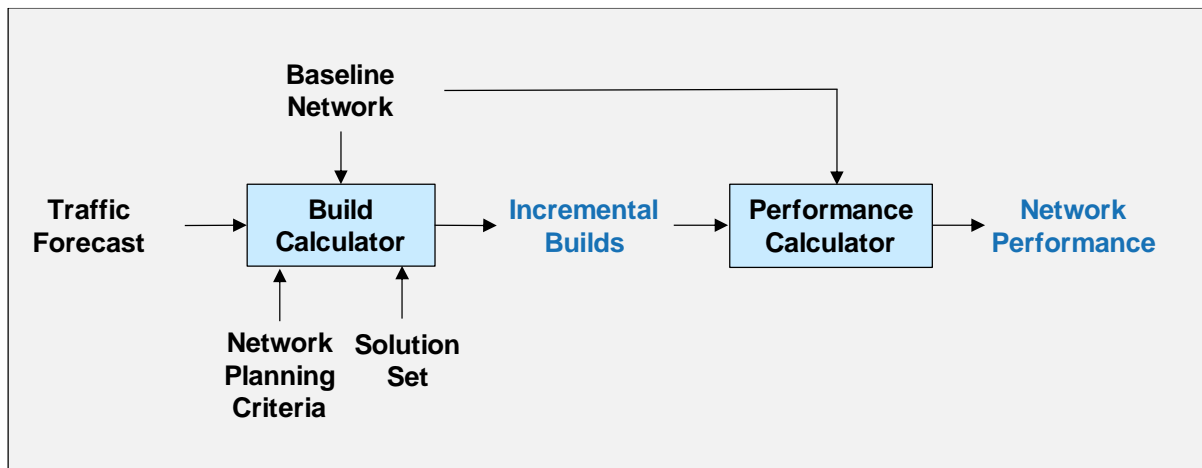
Figure 4: Schematic of Network Build Model
